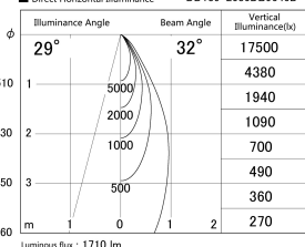
■ Direct Horizontal Illuminance DD139-2030DB9040D
