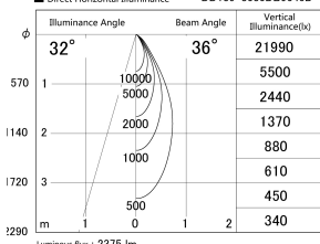
■ Direct Horizontal Illuminance DD139-3030DB9040D
