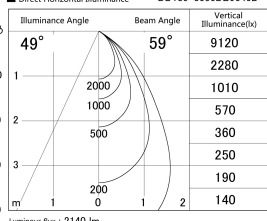
■ Direct Horizontal Illuminance DD139-3050DB9040D
