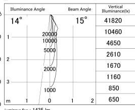
■ Direct Horizontal Illuminance DD139-1515WW9027D
