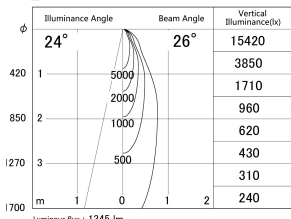
■ Direct Horizontal Illuminance DD139-1520WW9027D
