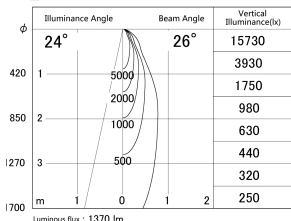
■ Direct Horizontal Illuminance DD139-1520WW9030D
