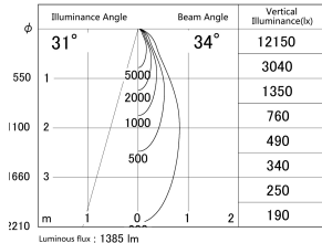
■ Direct Horizontal Illuminance DD139-1530WW9030D
