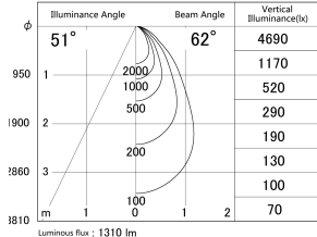
■ Direct Horizontal Illuminance DD139-1550WW9030D
