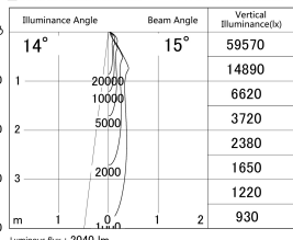
■ Direct Horizontal Illuminance DD139-2015WW9030D
