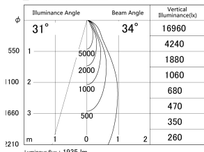
■ Direct Horizontal Illuminance DD139-2030WW9030D
