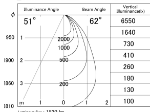
■ Direct Horizontal Illuminance DD139-2050WW9030D
