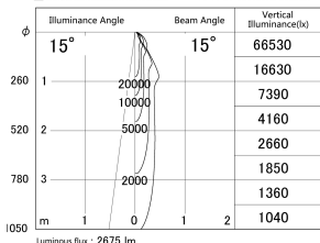
■ Direct Horizontal Illuminance DD139-3015WW9030D
