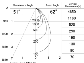
■ Direct Horizontal Illuminance DD139-1550WW9035D
