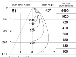
■ Direct Horizontal Illuminance DD139-2050WW9035D
