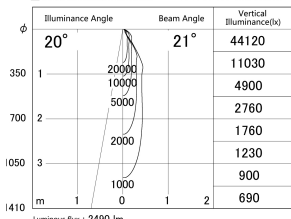
■ Direct Horizontal Illuminance DD139-2520WW9035D
