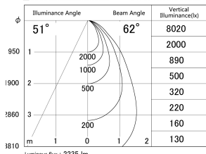
■ Direct Horizontal Illuminance DD139-2550WW9035D
