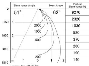
■ Direct Horizontal Illuminance DD139-3050WW9035D
