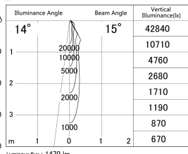
■ Direct Horizontal Illuminance DD139-1515WW9040D
