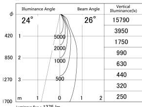
■ Direct Horizontal Illuminance DD139-1520WW9040D
