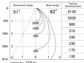
■ Direct Horizontal Illuminance DD139-2550WW9040D
