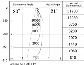
■ Direct Horizontal Illuminance DD139-3020WW9040D
