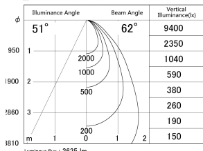
■ Direct Horizontal Illuminance DD139-3050WW9040D
