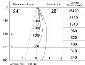
■ Direct Horizontal Illuminance DD139-1520WB9027D
