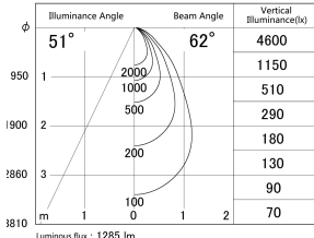
■ Direct Horizontal Illuminance DD139-1550WB9027D
