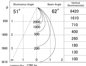
■ Direct Horizontal Illuminance DD139-2050WB9027D
