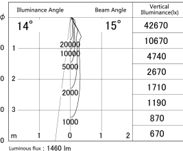
■ Direct Horizontal Illuminance DD139-1515WB9030D
