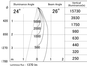
■ Direct Horizontal Illuminance DD139-1520WB9030D
