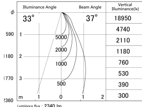
■ Direct Horizontal Illuminance DD139-2530WB9030D
