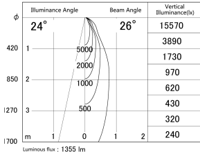
■ Direct Horizontal Illuminance DD139-1520WB9035D
