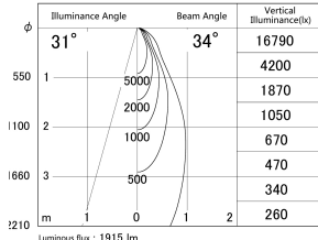
■ Direct Horizontal Illuminance DD139-2030WB9035D
