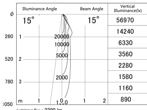
■ Direct Horizontal Illuminance DD139-2515WB9035D
