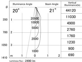
■ Direct Horizontal Illuminance DD139-2520WB9035D
