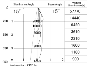
■ Direct Horizontal Illuminance DD139-2515WB9040D
