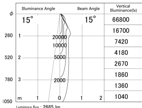
■ Direct Horizontal Illuminance DD139-3015WB9040D
