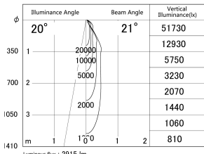
■ Direct Horizontal Illuminance DD139-3020WB9040D
