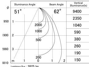
■ Direct Horizontal Illuminance DD139-3050WB9040D
