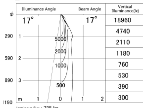
■ Direct Horizontal Illuminance DD140-0815MW9027D
