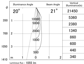
■ Direct Horizontal Illuminance DD140-1020MW9027D
