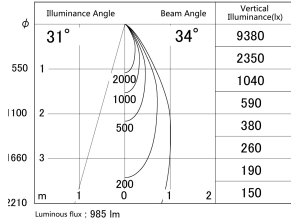
■ Direct Horizontal Illuminance DD140-1030MW9027D
