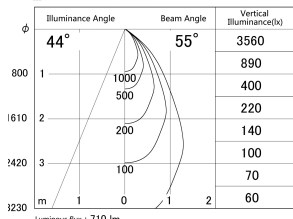
■ Direct Horizontal Illuminance DD140-0850MW9030D
