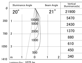
■ Direct Horizontal Illuminance DD140-1020MW9030D
