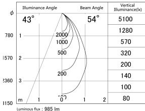
■ Direct Horizontal Illuminance DD140-1050MW9030D
