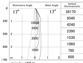
■ Direct Horizontal Illuminance DD140-1515MW9030D
