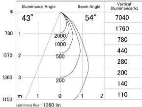
■ Direct Horizontal Illuminance DD140-1550MW9030D
