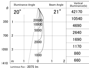
■ Direct Horizontal Illuminance DD140-2020MW9030D
