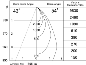
■ Direct Horizontal Illuminance DD140-2050MW9030D
