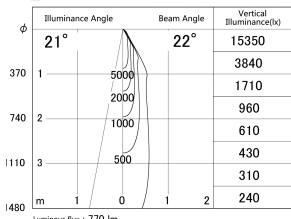
■ Direct Horizontal Illuminance DD140-0820MW9035D
