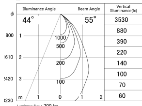
■ Direct Horizontal Illuminance DD140-0850MW9035D
