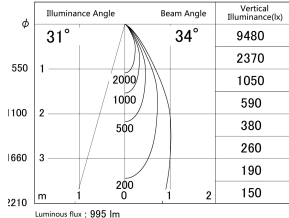
■ Direct Horizontal Illuminance DD140-1030MW9035D
