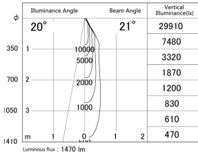
■ Direct Horizontal Illuminance DD140-1520MW9035D
